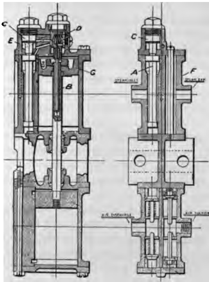
FIG. 380.—Sectional View of the Valve Motion and Mechanism of the "Victor" Auxiliary Steam Pumps.
